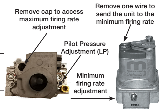
Fig. 2 Separate Regulator and Modulating Valves
