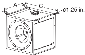
Horizontal Hanging Neoprene Mount
