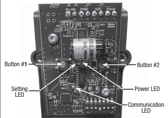
EXA Modulating Gas Valve (with cover removed)
