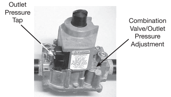
Combined Regulator Valve
